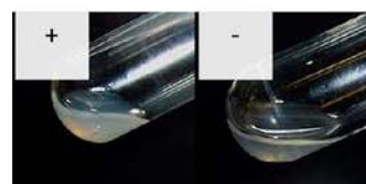
Tube Coagulase
