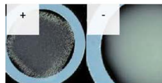
Slide Coagulase
